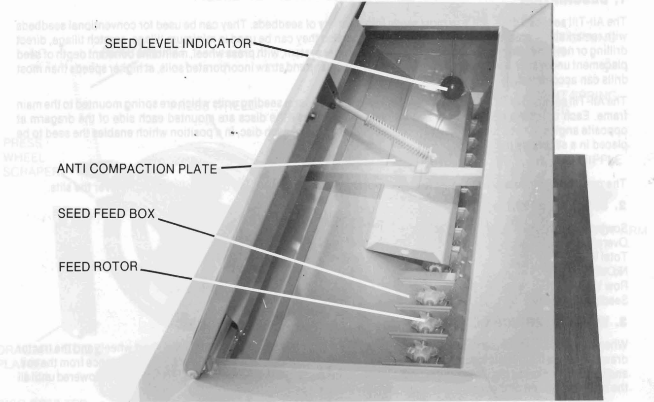
FIGURE 1. DRAG ARM SEEDING UNIT
